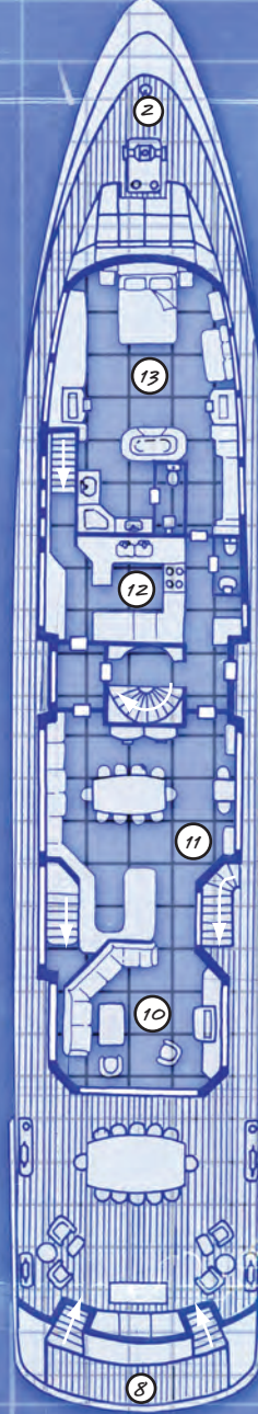
MAIN DECK
